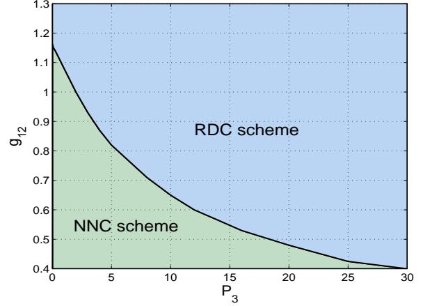
Fig. 3. Regions for the preferred coding scheme (the proposed RDC or NNC) versus P_3 and g_{12} where g_{13} = g_{23} = 1 and P_1 = P_2 = 2 .
